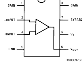
Dual-In-Line and Small Outline Packages
