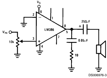
Amplifier with Gain = 200 Minimum Parts
