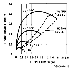
Device Dissipation vs Output Power—16 \Omega Load
